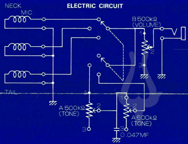
ELECTRIC CIRCUIT
